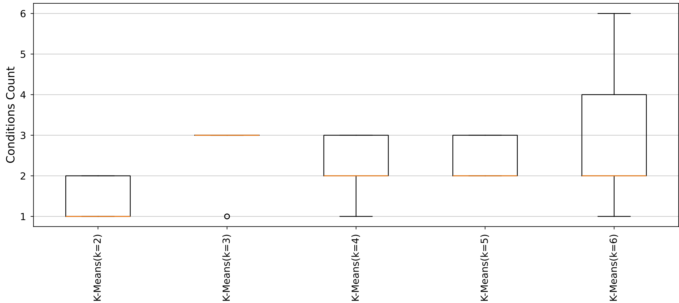
YARA Rules Conditions Count Distribution (Cluster23_Size6 dataset)
